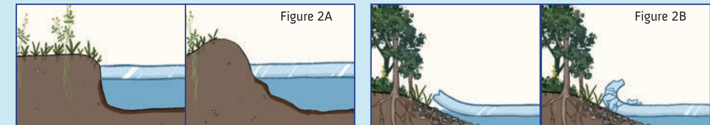
Figures 2A and 2B: Showing ice push and break up along a shoreline.
