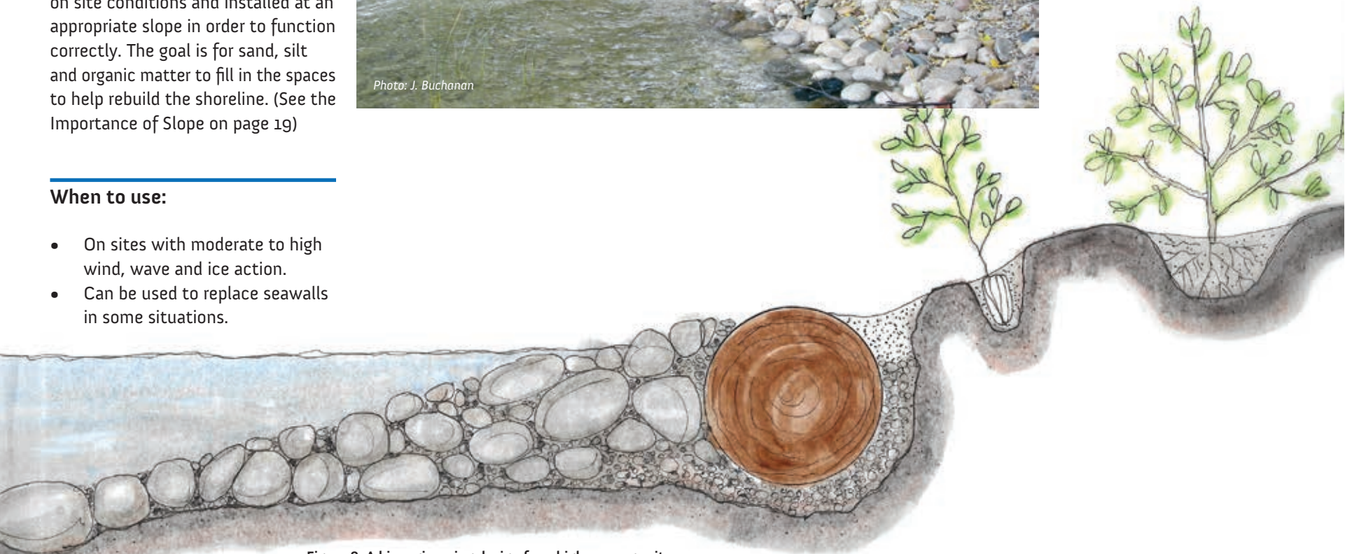
Figure 8: A bioengineering design for a higher energy site.
